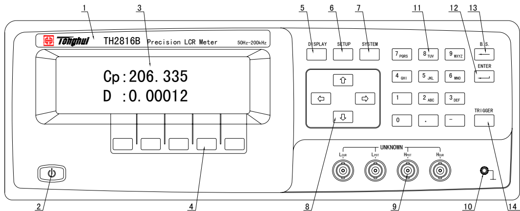
Figure 3-1. Front panel overview
