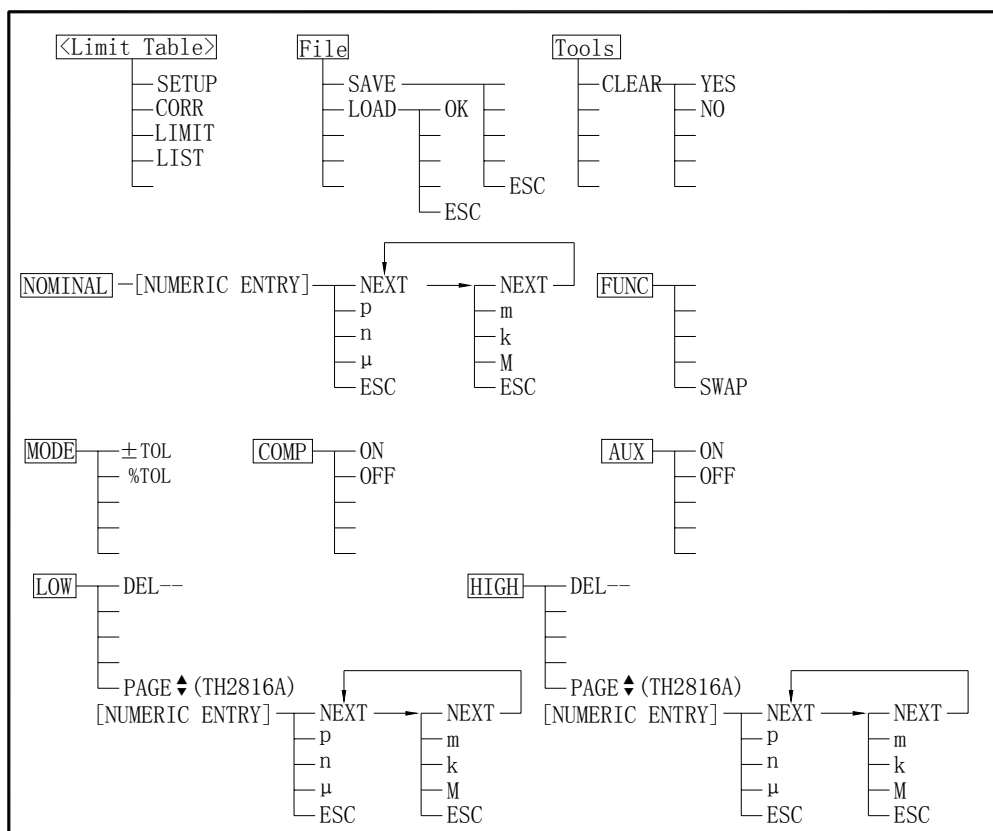
Figure 4-15. Available Softkeys on the Limit Table Page
